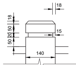
POST TOP DETAIL
