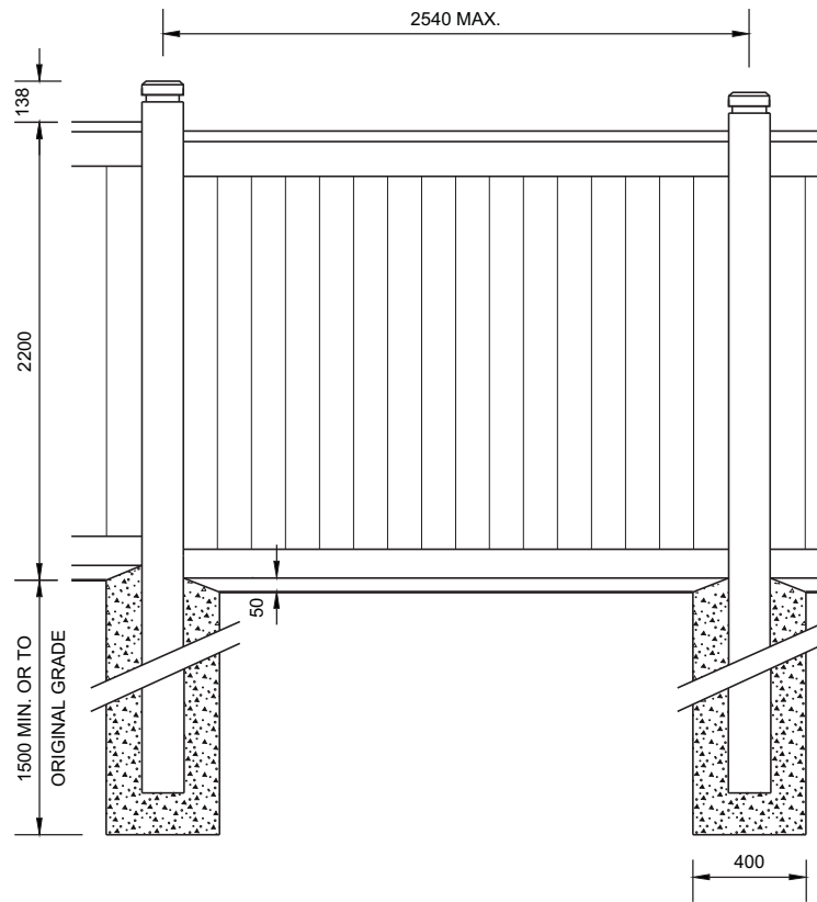
FRONT ELEVATION
