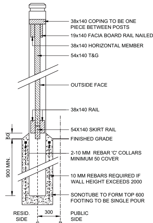
TYPICAL SECTION
